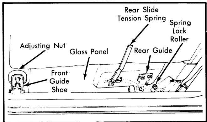
Fig. 2 Front Guide Shoe and Rear Tension Spring
