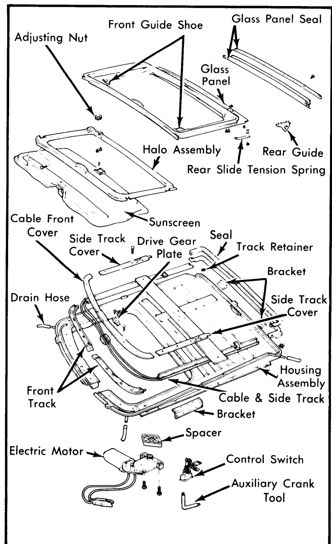
Fig. 1 Exploded View of Jeep Power Sunroof Assembly
