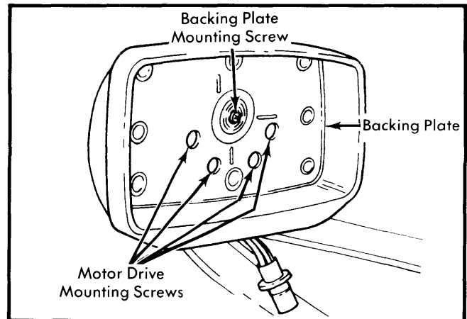
Fig. 1 Electric Mirror Mounting Screws
