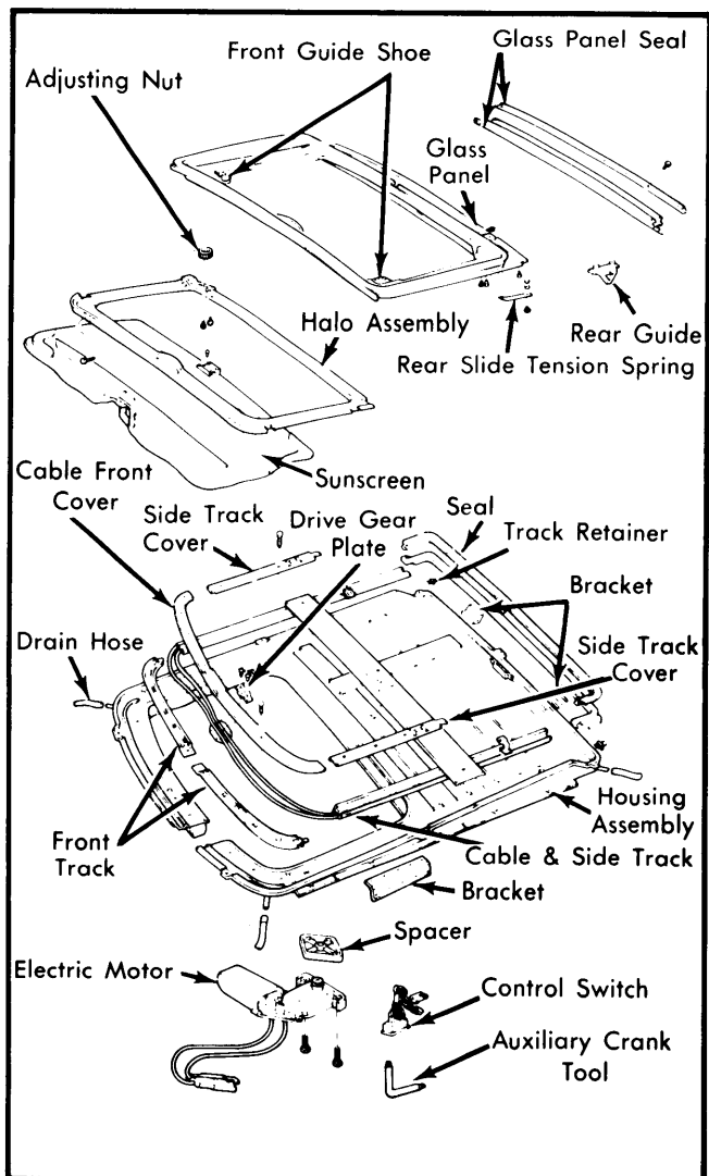
Fig. 1 Exploded View of Jeep Power Sunroof Assembly
