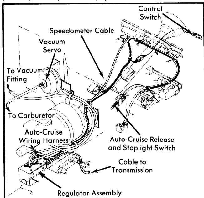
Fig. 1 IHC Auto-Cruise System
