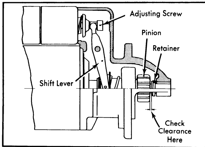
Fig. 2 Checking Pinion Clearance
