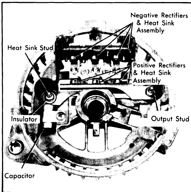
Fig. 4 View Rectifier End Shield
