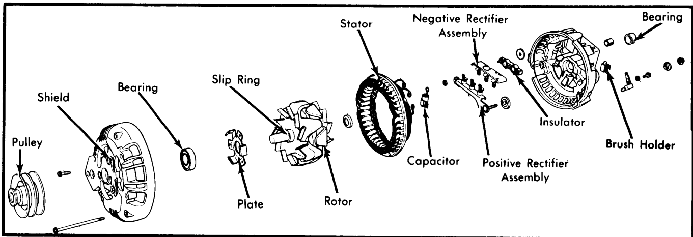
Fig. 6 Exploded View of Typical Chrysler Corp. Alternator
