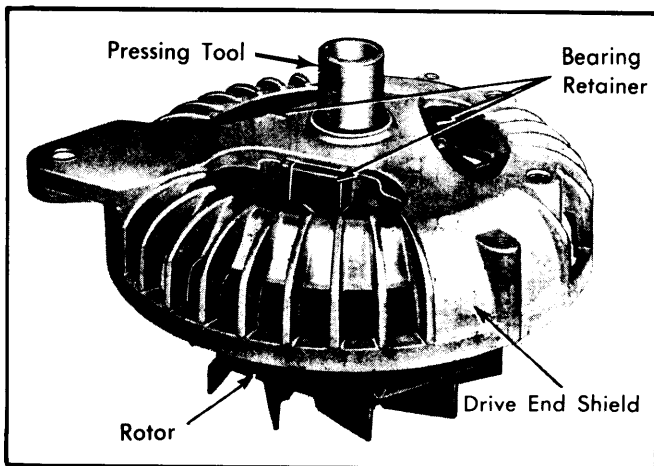
Fig. 5 Installing Drive End Shield Bearing
