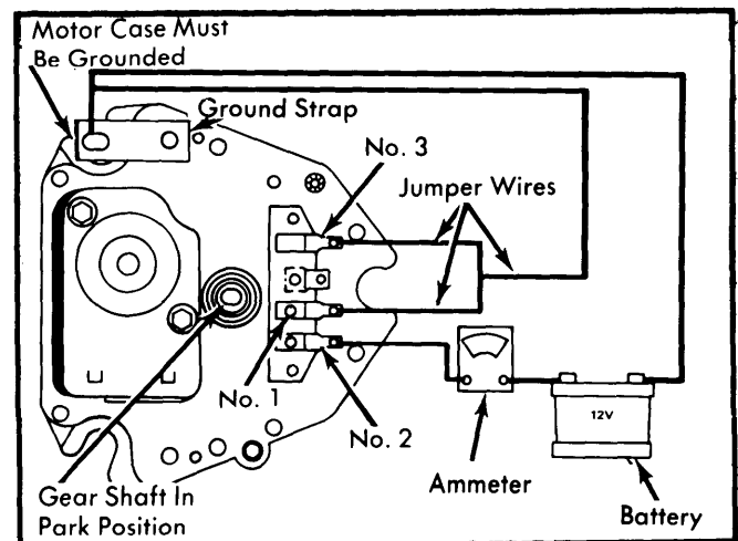
Fig. 4 Jeep Identification of Test Connections (Cherokee, Wagoneer & "J" Models)
