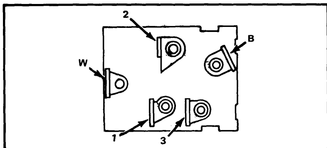
Fig. 2 Jeep Identification of Test Connections
