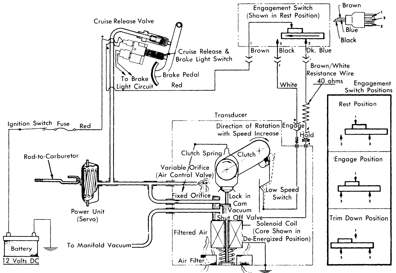
Fig. 1 General Motors Cruise Master Speed Control Wiring & Pneumatic Diagram
