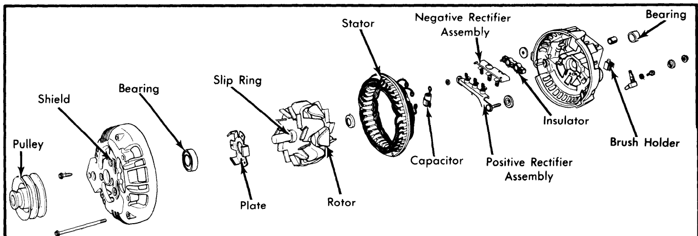
Fig. 6 Exploded View of Chrysler Corp. Alternator
