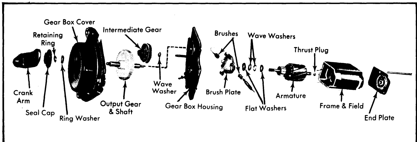
Fig. 3 Exploded View of Wiper Motor & Drive Assembly
