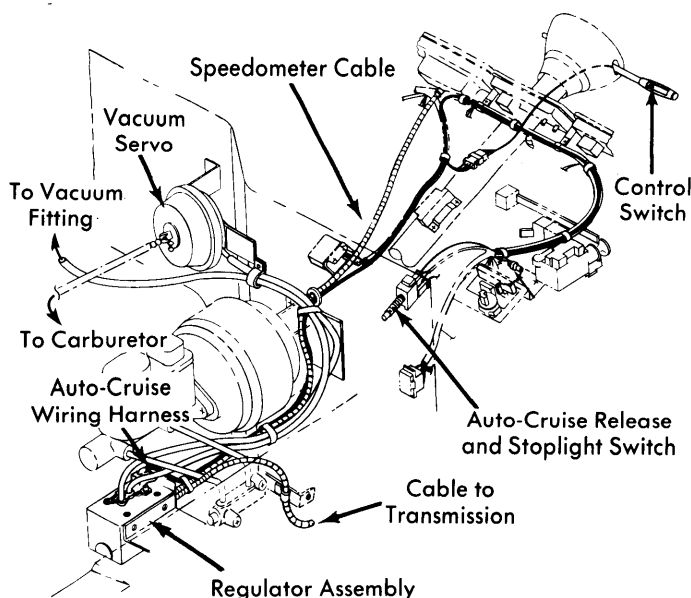
Fig. 1 IHC Auto-Cruise System
