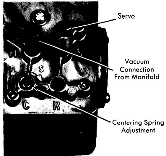
Fig. 3 IHC Centering Spring Adjustment Screw
