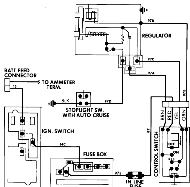
Fig. 2 IHC Auto-Cruise System Wiring Diagram
