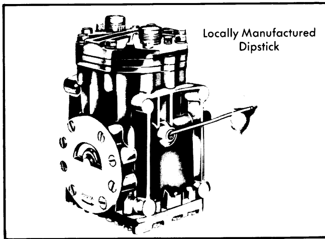
Fig. 4 Checking Oil Level On Vertically Mounted York Compressor
