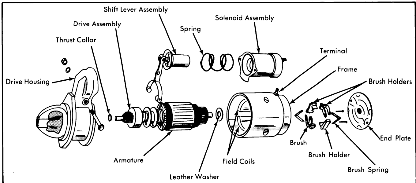
Fig. 6 Exploded View of Delco-Remy Enclosed Housing Starter Assembly
