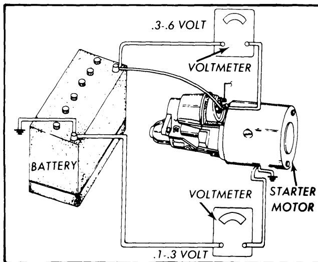
VOLTAGE-DROP TEST
