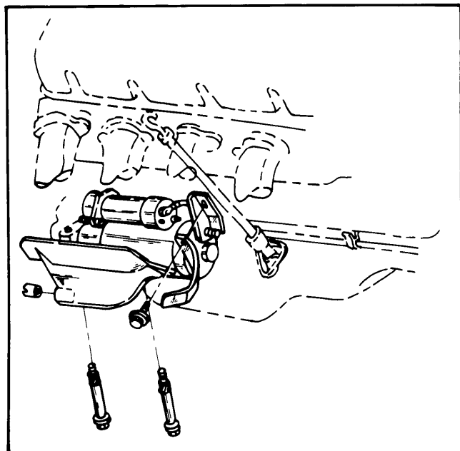
STARTER & HEAT SHIELD INSTALLATION (TYPICAL)
