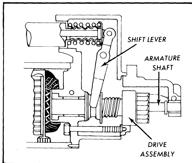
ARMATURE SHAFT & DRIVE ASSEMBLY
