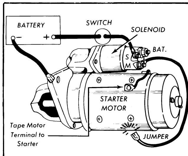
SOLENOID PULL-IN WINDING TEST
