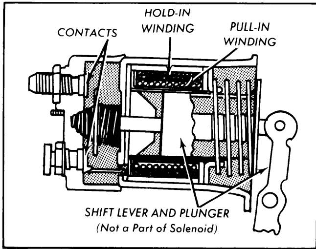
SOLENOID ASSEMBLY
