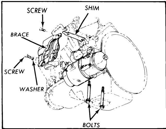
STARTER SHIM INSTALLATION (TYPICAL)
