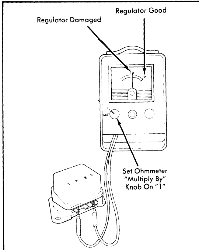
Fig. 2 Test Connections for Burned or Open Connector Wire
