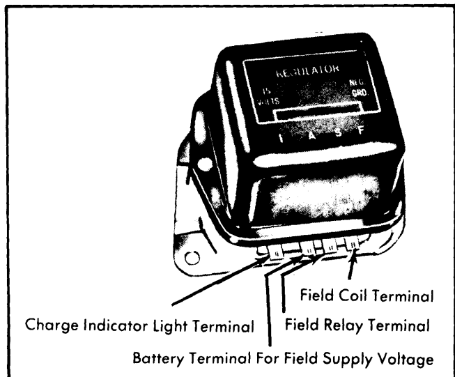
Fig. 1 Identifying Regulator Terminals
