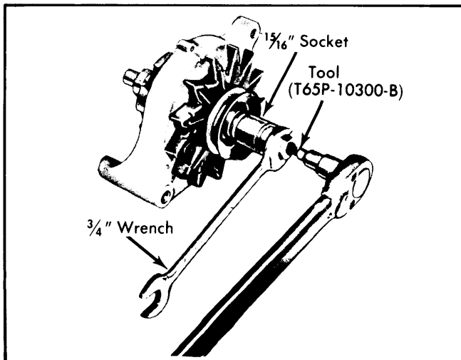
Fig. 7 View Showing Alternator Pulley Removal Procedure
