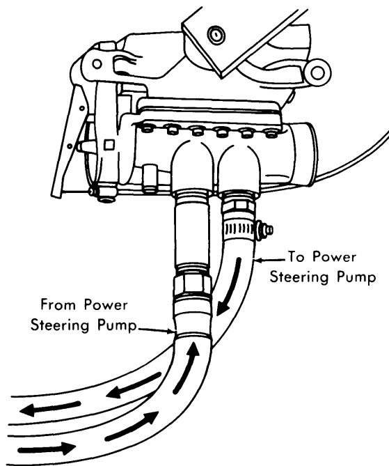
Fig. 1 Inlet & Outlet Connections for Wiper Motor Hoses
