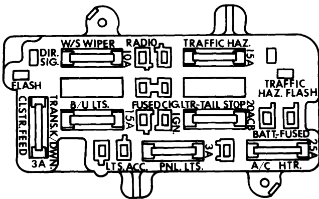
Fig. 1 "CJ" Models Fuse Panel
