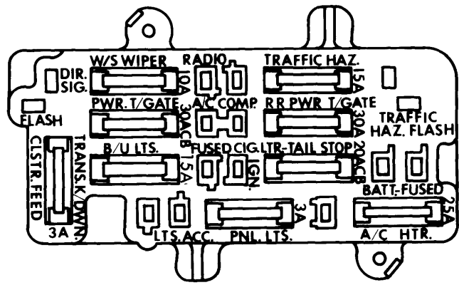
Fig. 2 All Models (Exc. "CJ") Fuse Panel
