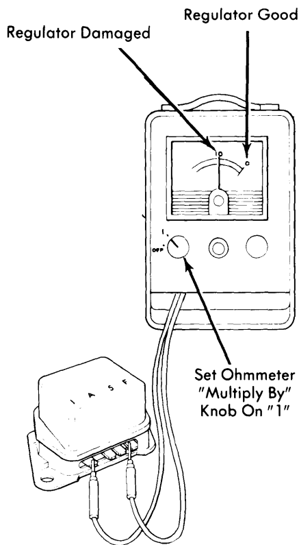
Fig. 2 Test Connections for Burned or Open Connector Wire
