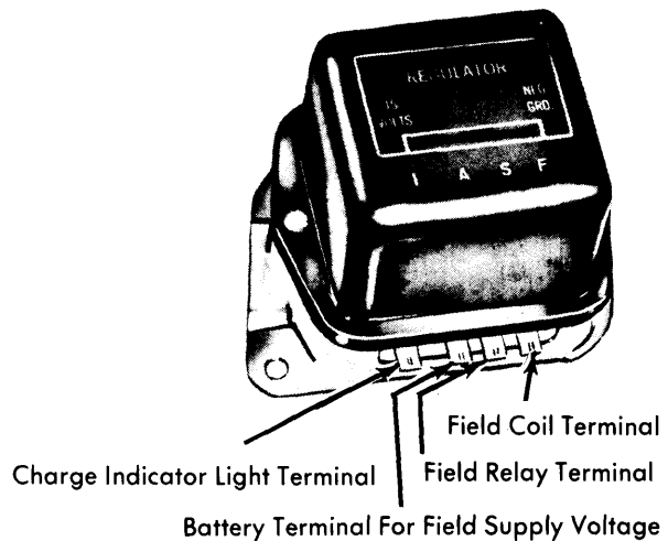
Fig. 1 Identifying Regulator Terminals
