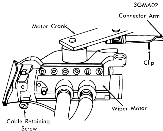
REMOVING LINKAGE
