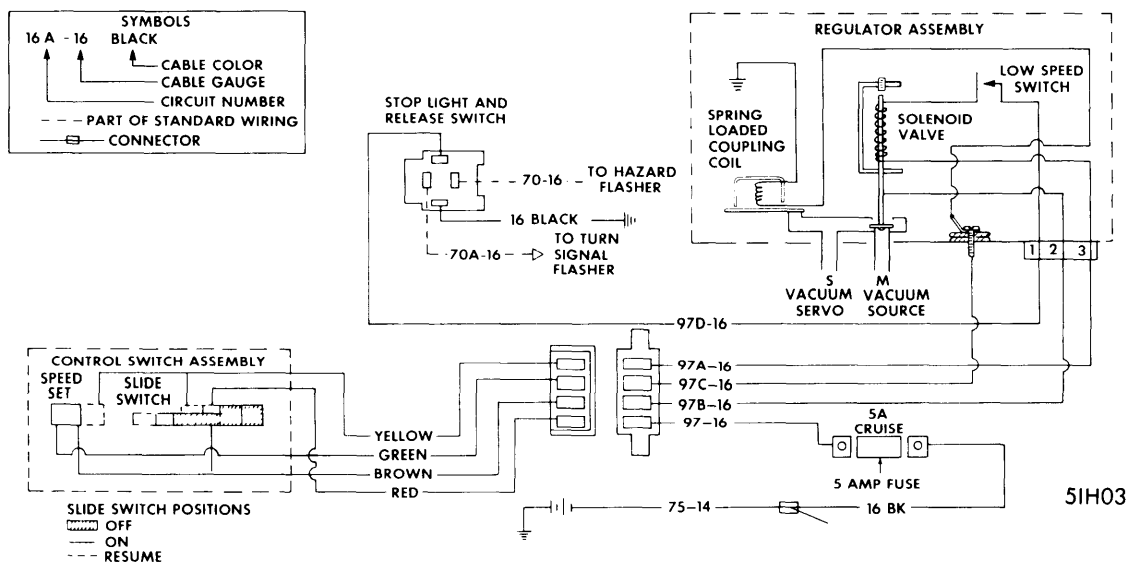
AUTO-CRUISE WIRING DIAGRAM
