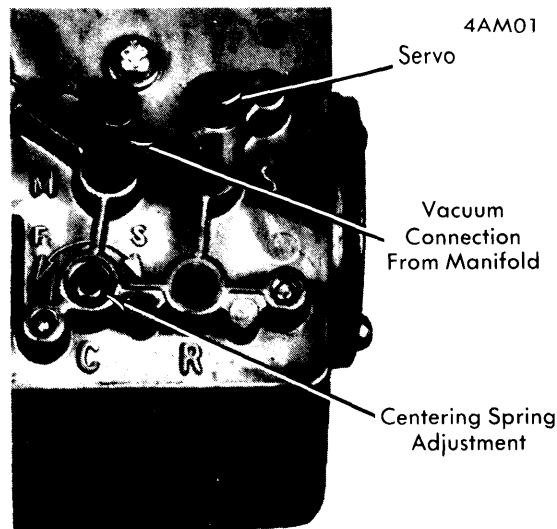
ADJUSTMENT SCREW IDENTIFICATION
