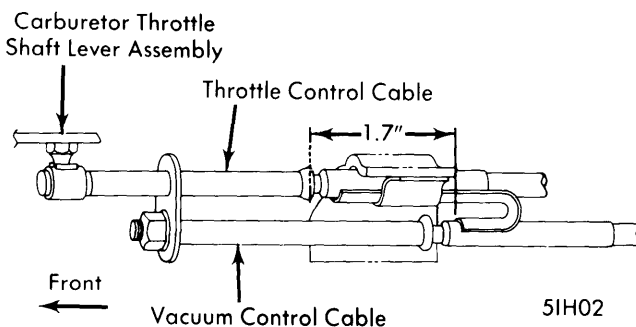
VACUUM CONTROL CABLE ADJUSTMENT
