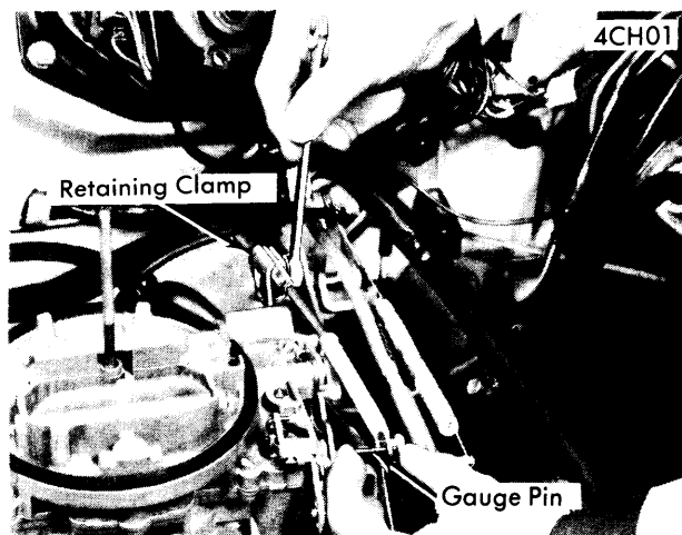
SERVO THROTTLE CABLE ADJUSTMENT
