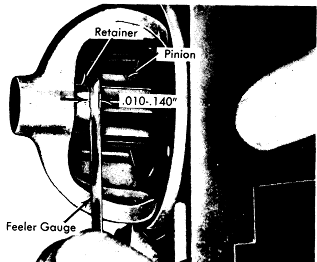
CHECKING PINION END PLAY
