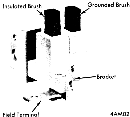
BRUSH ASSEMBLY TEST
