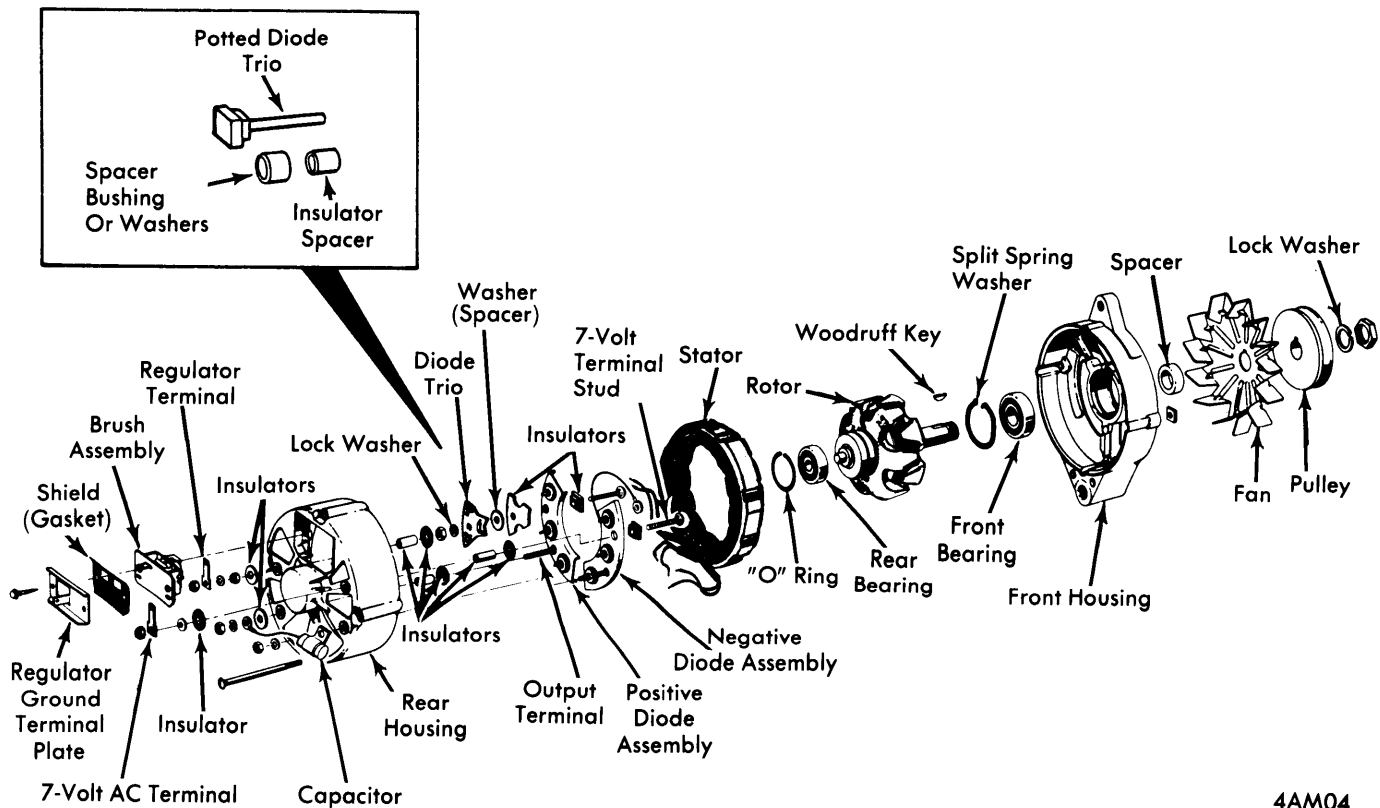
DISASSEMBLED ALTERNATOR
