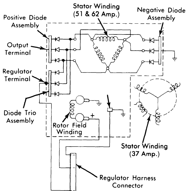
4AM01 ALTERNATOR CIRCUIT
