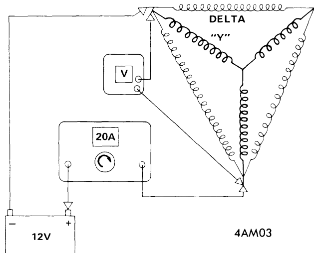
STATOR LOAD TEST
