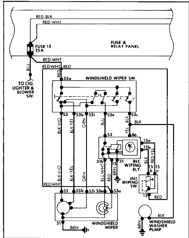
Fig. 2: 924 & 924 Turbo Wiper System Wiring Diagram
