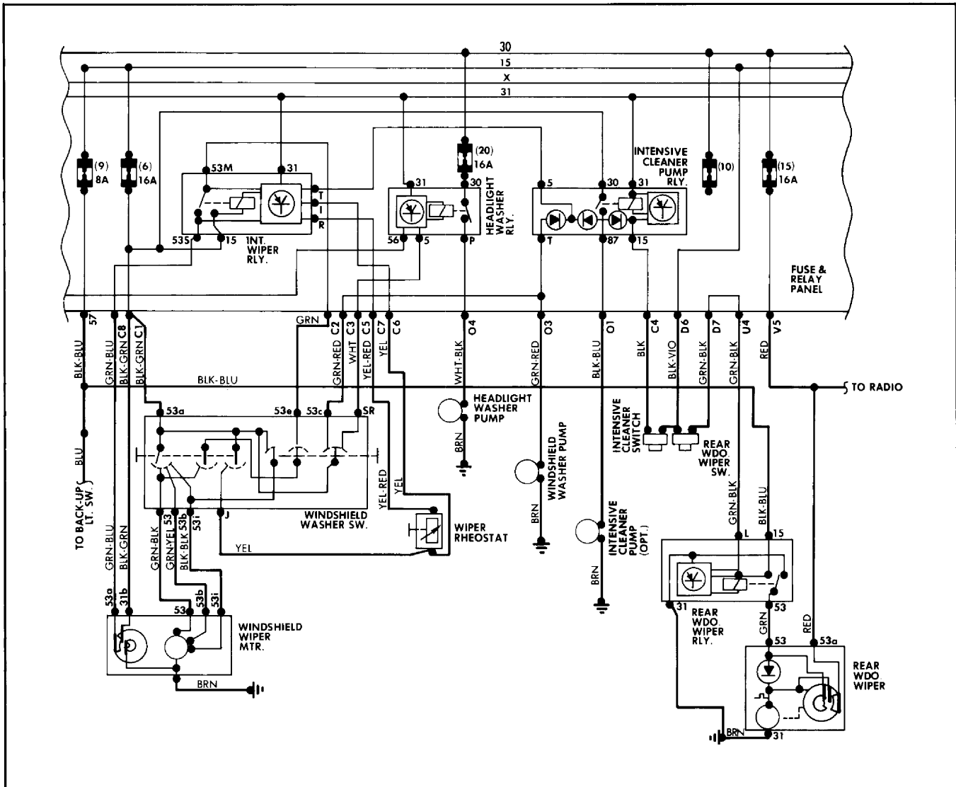
Fig. 3: 928 Wiper System Wiring Diagram
