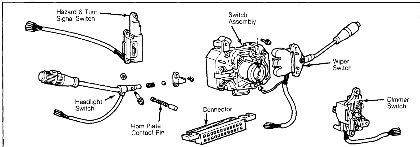
Fig. 1 Exploded View of Combination Switch
