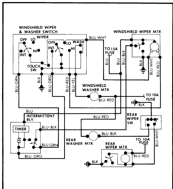
Fig. 1 Mazda GLC Hatchback Wiring Diagram
