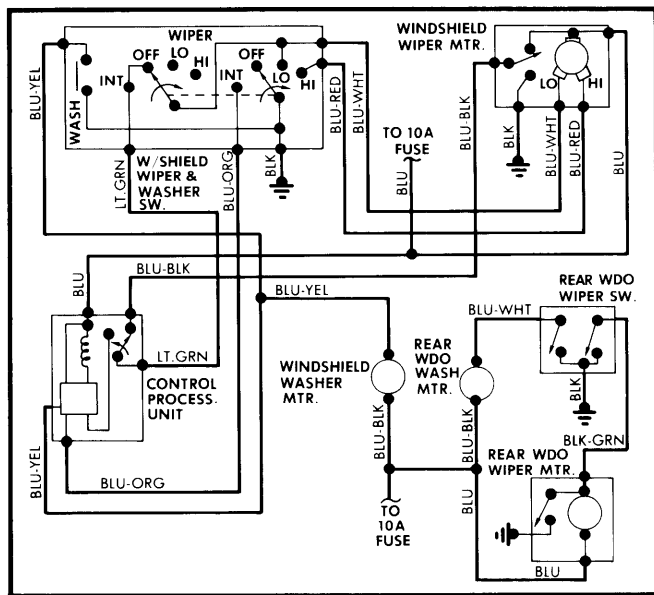
Fig. 3 Mazda RX7 Wiring Diagram
