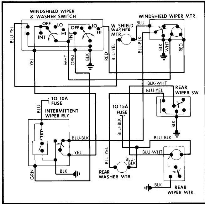
Fig. 2 Mazda GLC Wagon Wiring Diagram
