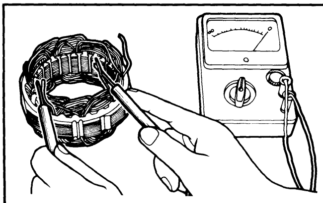
Fig. 2 Stator Coil Continuity Test
