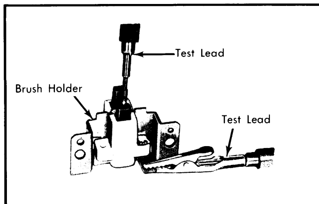
Fig. 3 Checking Brush Holder
