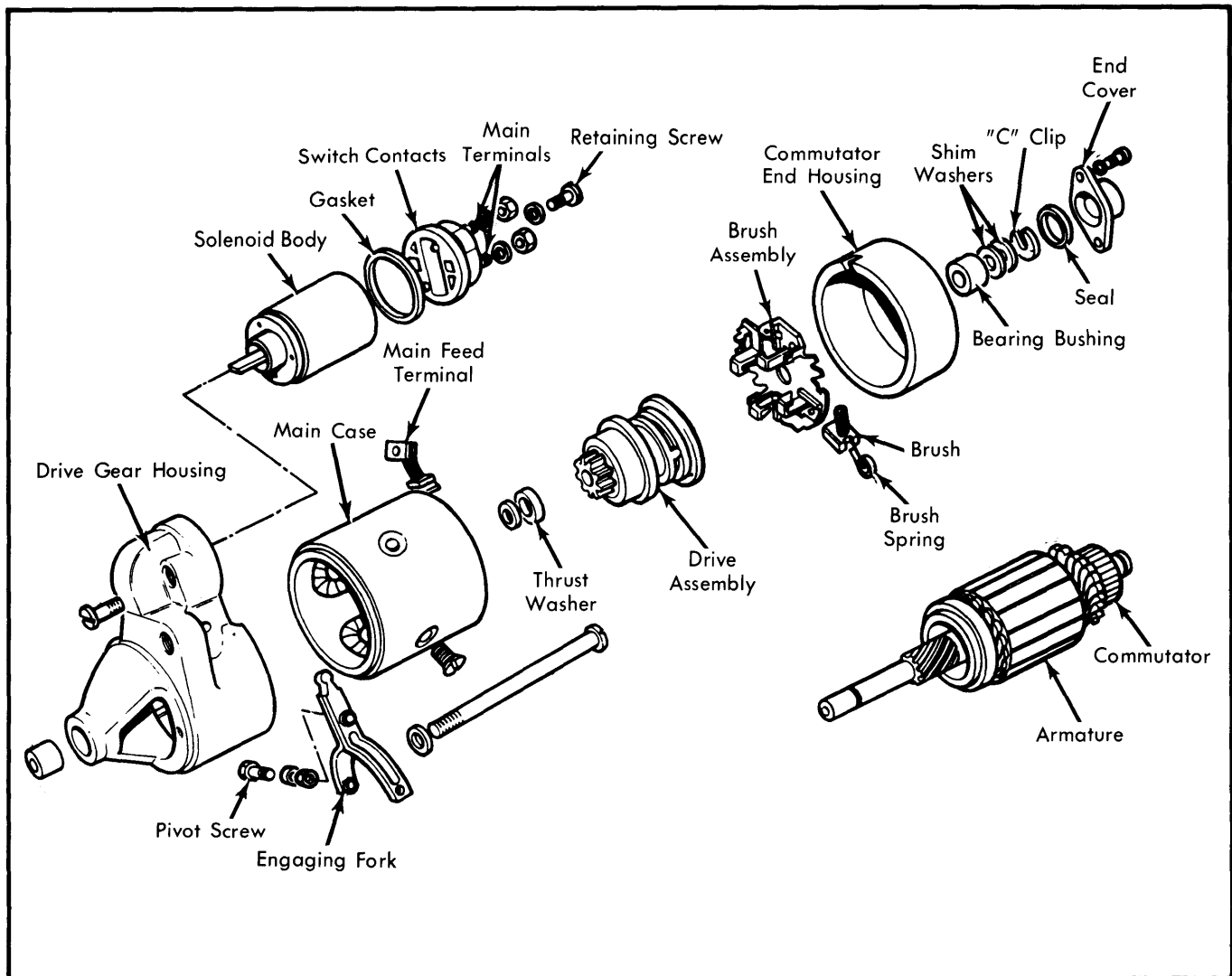
Fig. 1 Disassembled View of Typical Bosch Starter
