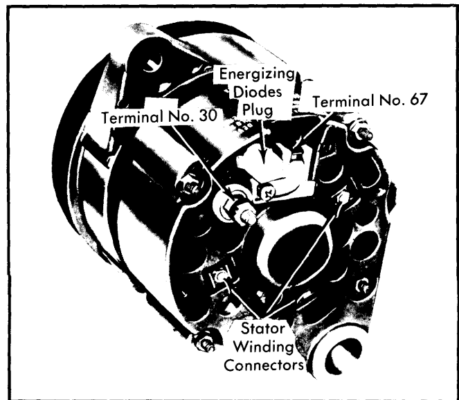
Fig. 1 Marelli Alternator Test Points
