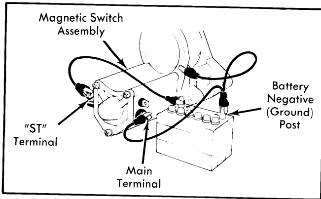
Fig. 2 Magnetic Switch Pull-In Coil Hook-Up
