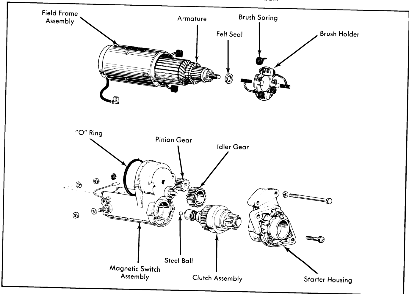
Fig. 4 Exploded View of Nippondenso Reduction Gear Starter
