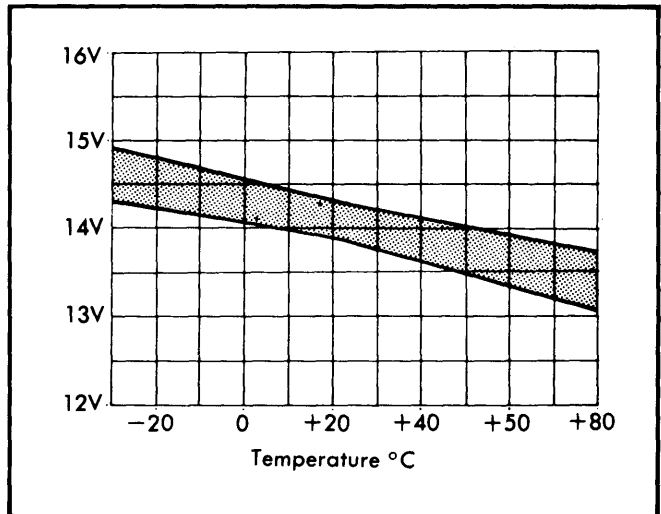
Fig. 2 Voltage-Temperature Variation with Regulator Warm.
