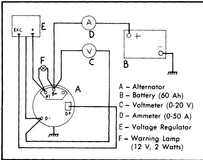
Fig. 1 Regulator Test Circuit
