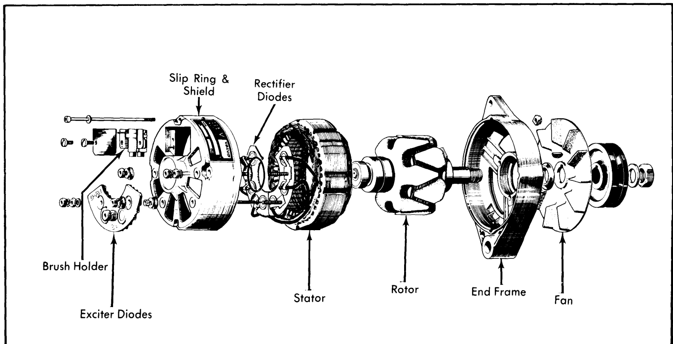
Fig. 1 Exploded View of Alternator
