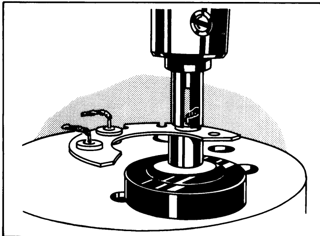
Fig. 3 Installing Diodes
