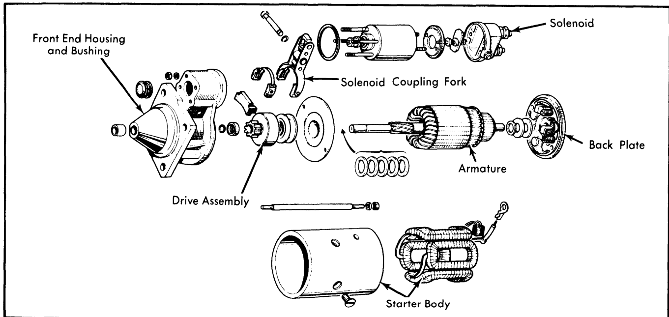
Fig. 1 Disassembled View of Paris Rhone Starter
