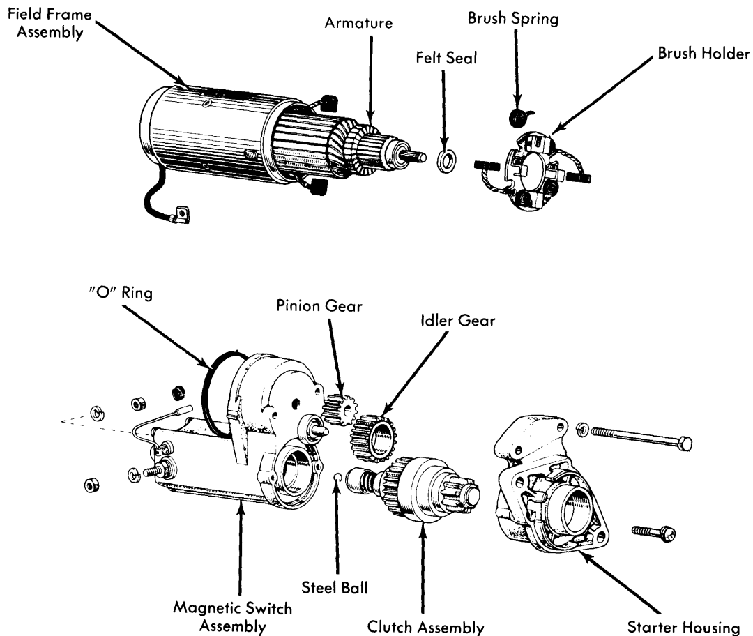
Fig. 4 Exploded View of Nippondenso Reduction Gear Starter (Toyota Model for 20R Engine Shown, Others Similar)
