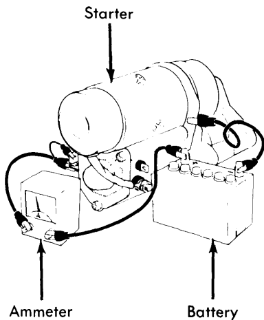
Fig. 1 Ammeter Hook-Up for No Load Test (Toyota Shown)
