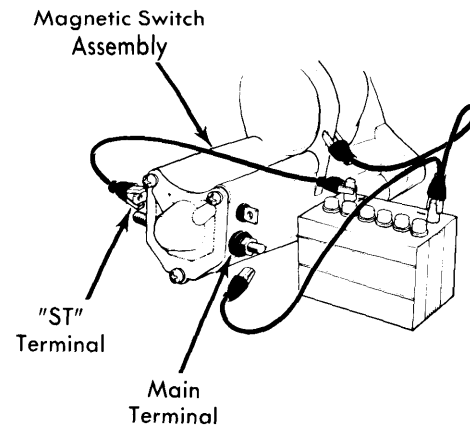
Fig. 3 Magnetic Switch Hold-In Test Hook-Up
