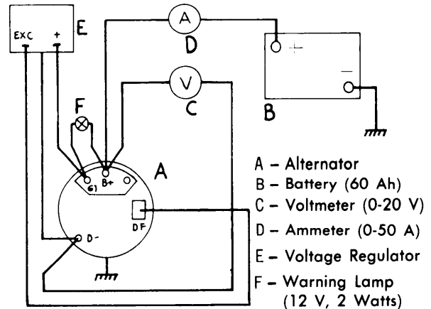
Fig. 1 Regulator Test Circuit
