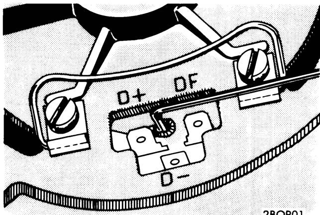
LIFTING CARBON BRUSHES (0 120 400 600 SERIES)
