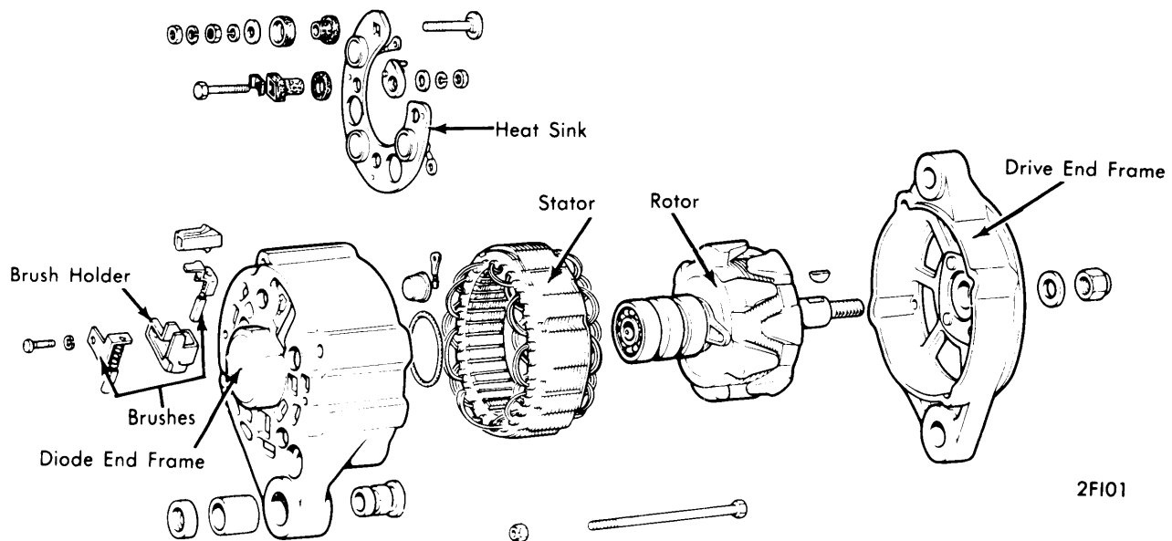
FIAT ALTERNATOR
