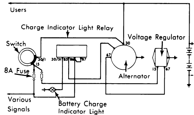
CHARGING WITH INDICATOR LIGHT (ONE POLE GROUNDED)
