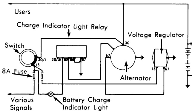
CHARGING WITH INDICATOR LIGHT (BOTH POLES GROUNDED)
