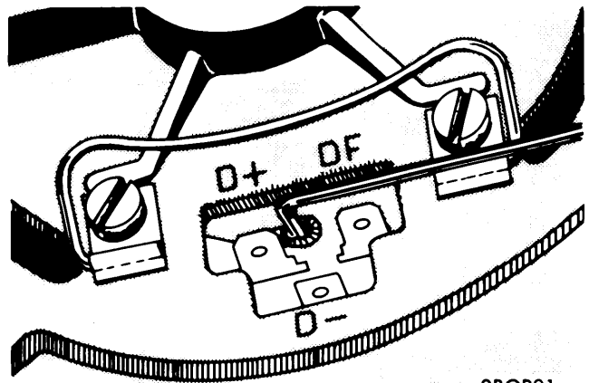
LIFTING CARBON BRUSHES (0 120 400 600 SERIES)
