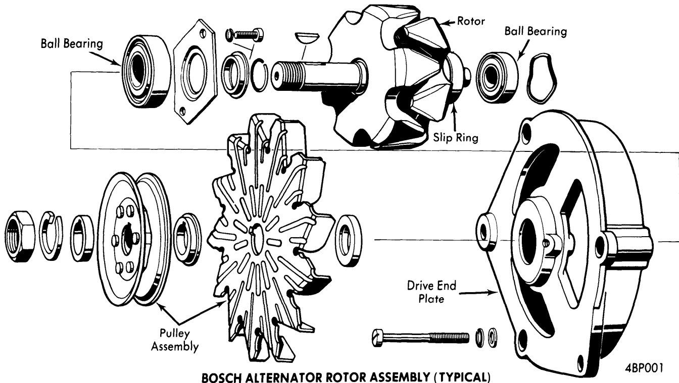
BOSCH ALTERNATOR ROTOR ASSEMBLY (TYPICAL)
