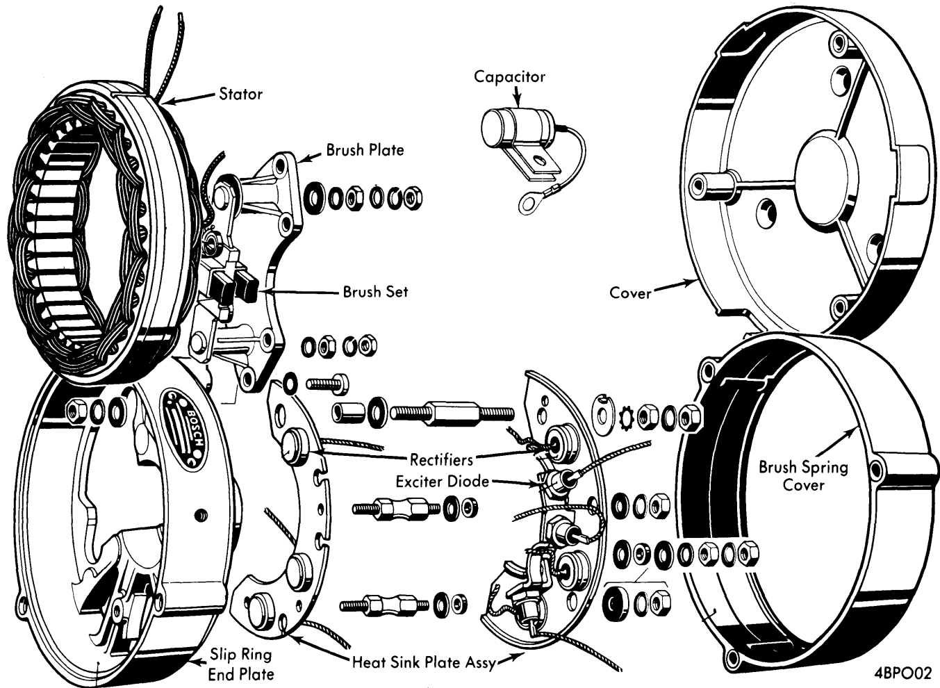
BOSCH ALTERNATOR FRAME ASSEMBLY (TYPICAL)
