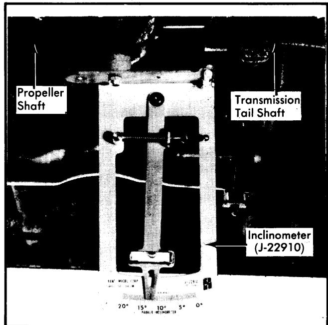
Fig. 2 Measuring Front Universal Joint Angle Using Pinion Angle Gauge (Inclinometer)
