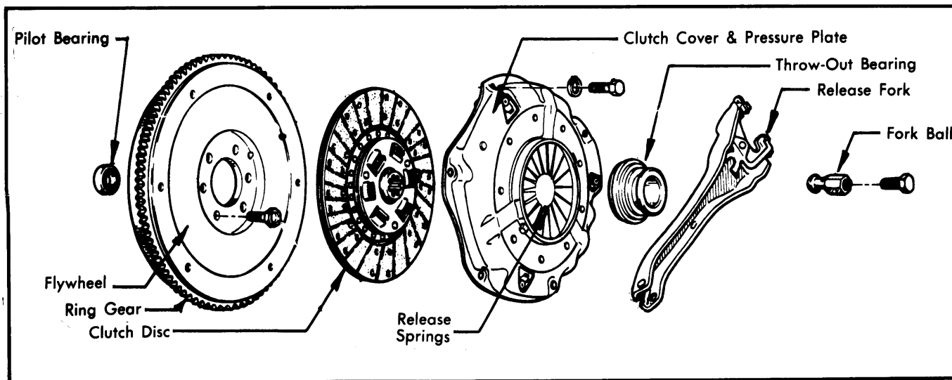
Fig. 1 Exploded View of Diaphragm Spring Clutch Assembly
