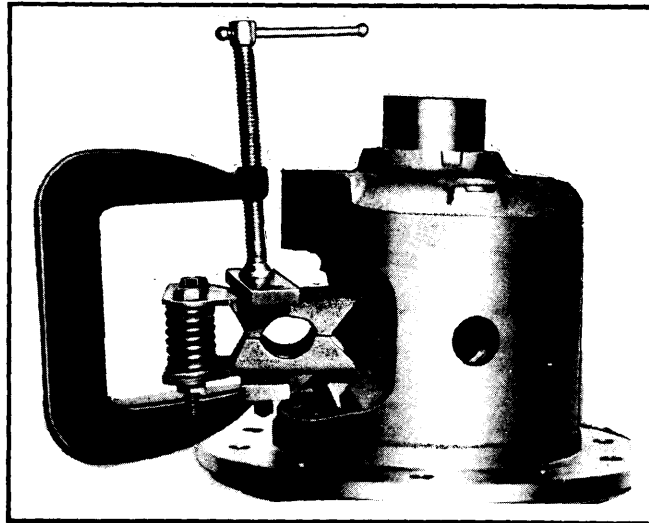
Fig. 2 Removing Preload Spring Pack (Coil Type Preload Spring)
