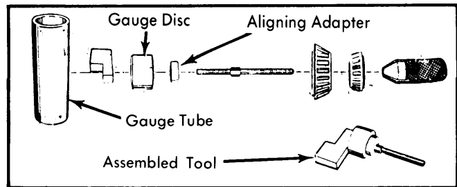
Fig. 4 Rear Axle Pinion Depth Gauge Tool Set
