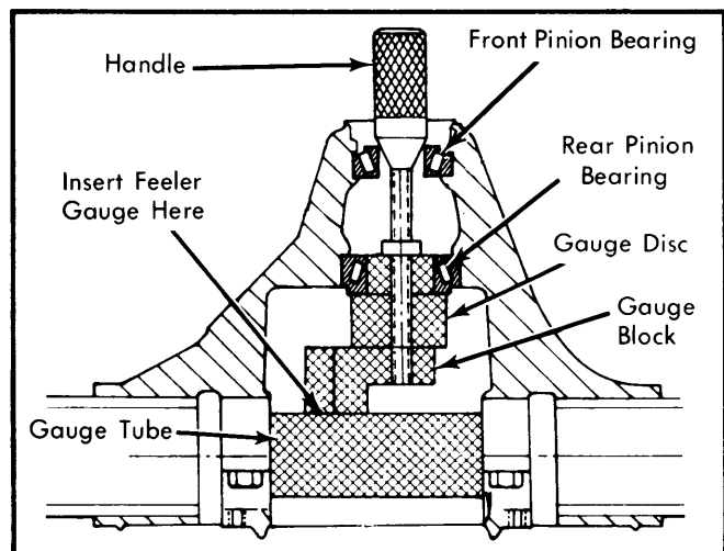
Fig. 5 Using Pinion Depth Gauge Tool
