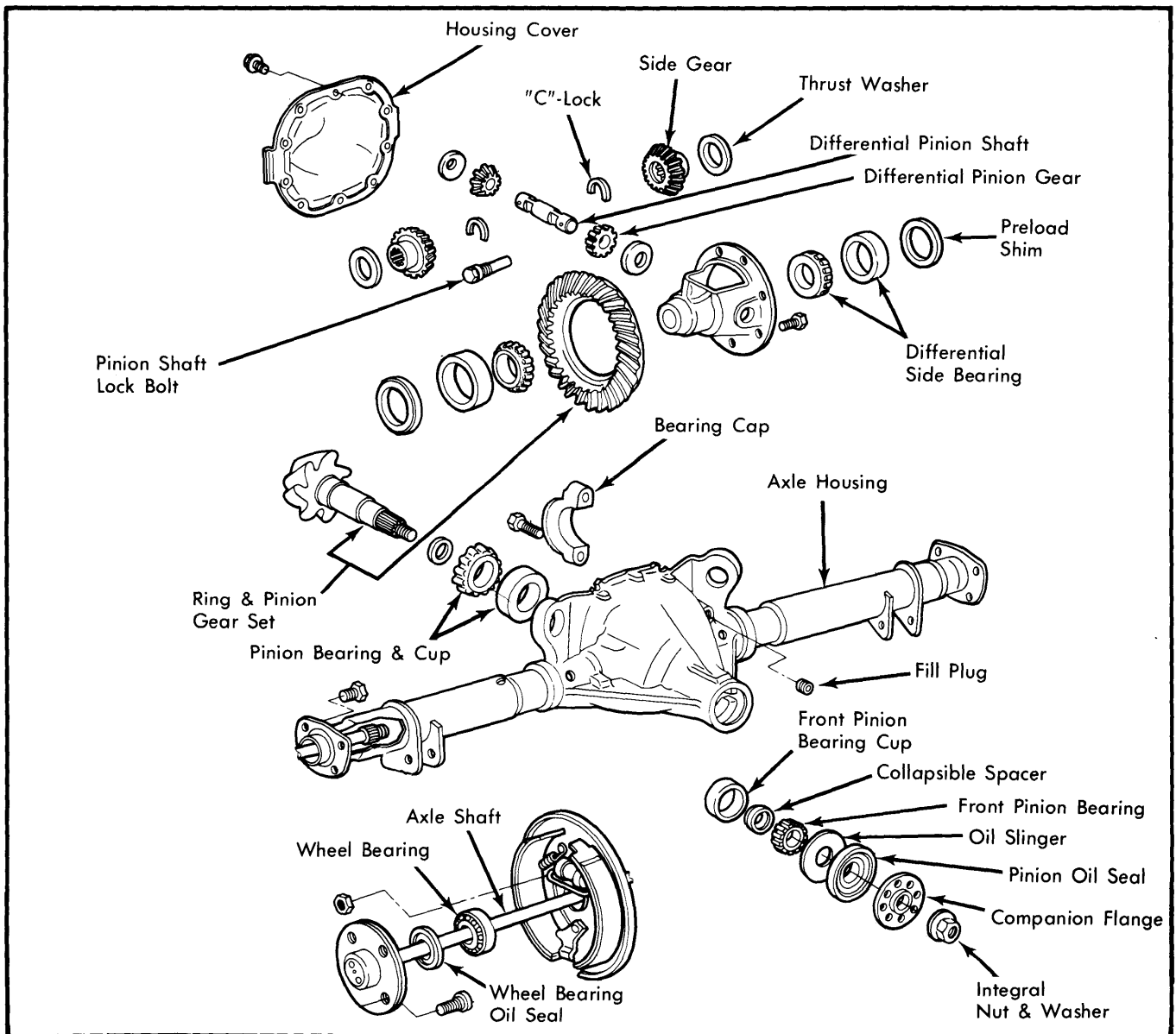
Fig. 2 Ford Motor Co. Integral Carrier Axle (WGX, WGY & WGZ Type)
