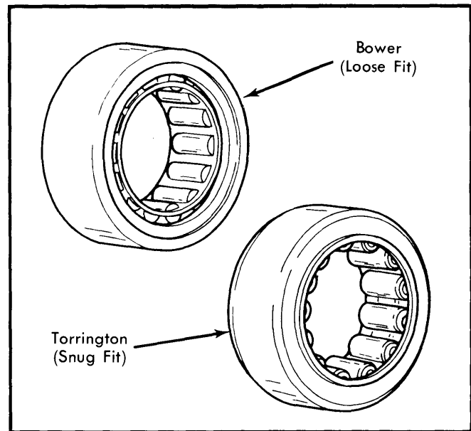
Fig. 3 Bower and Torrington Wheel Bearings
