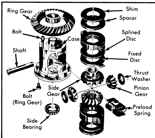
Fig. 1 Exploded View of Positraction Unit ("S" Shaped Preload Spring)
