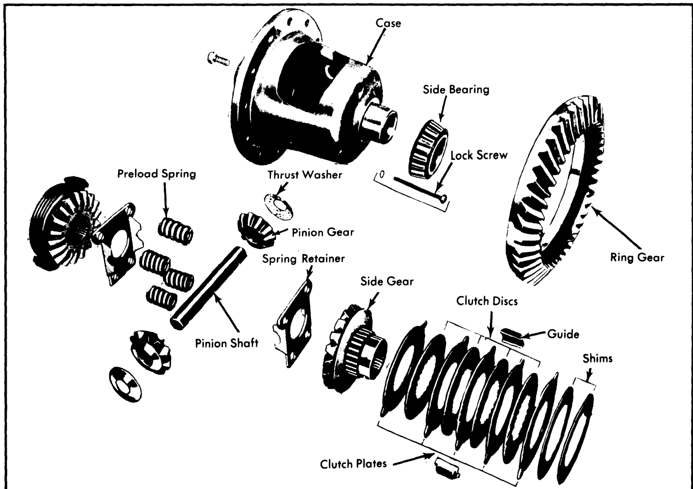
Fig. 3 Exploded View of Positraction Unit (Coil Type Preload Spring)
