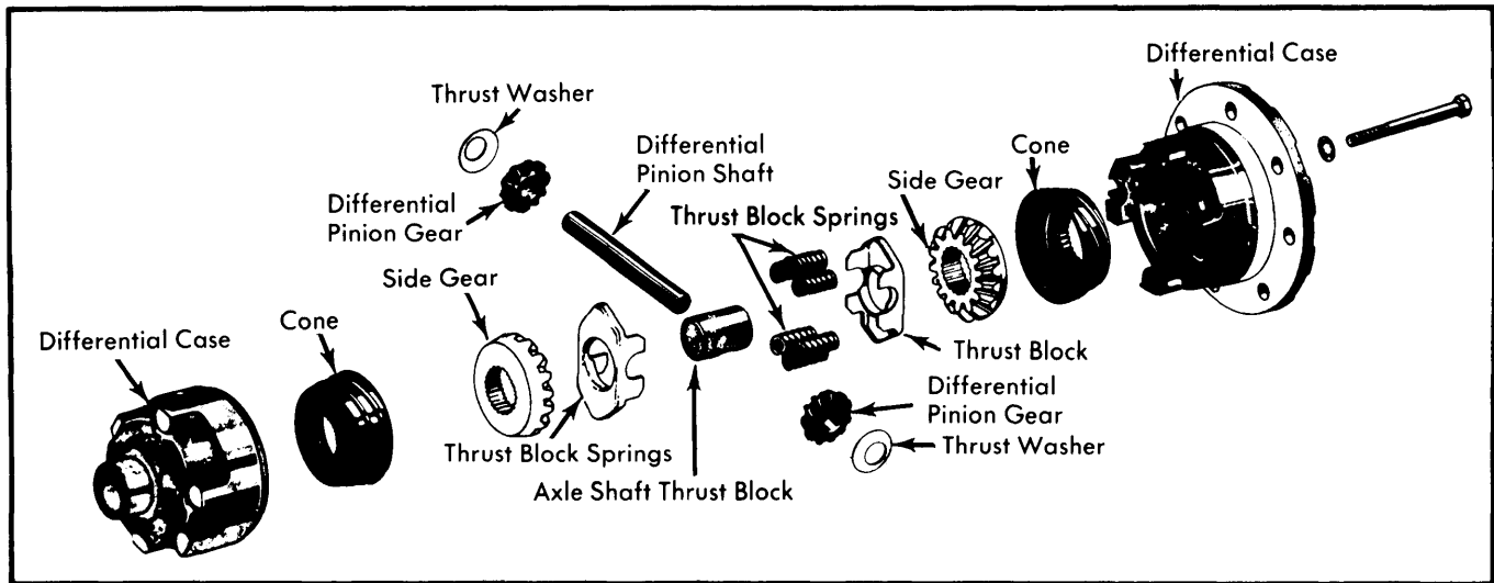
Fig. 1 American Motors 7 \frac{9}{16} " Twin Grip Differential
