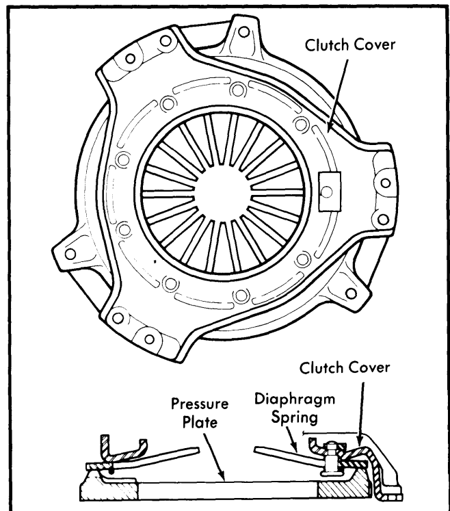
Fig. 3 American Motors 3-Bolt Clutch (All 6-Cyl. with 4-Speed Transmissions)
