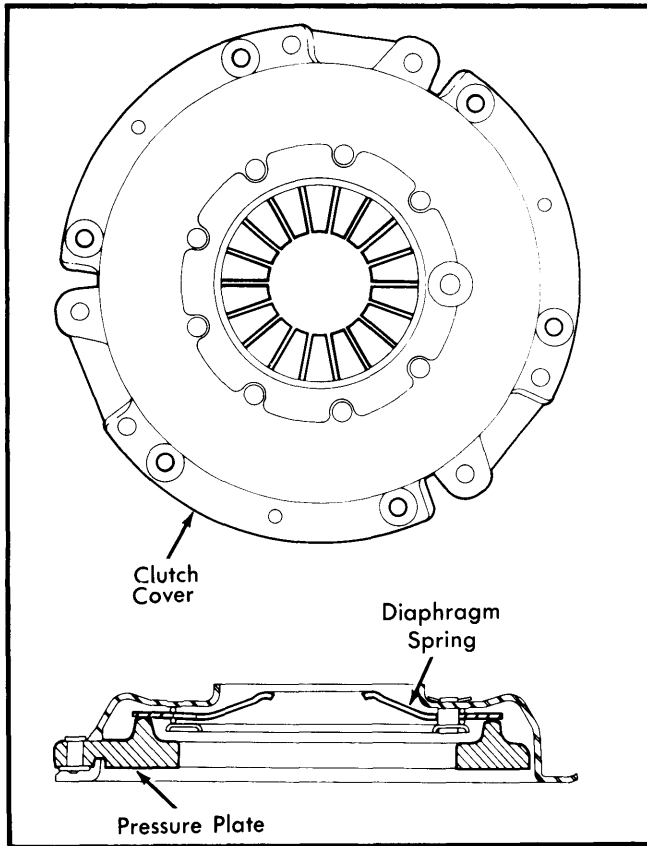
Fig. 4 American Motors 6-Bolt Clutch (All 4-Cyl. with 4-Speed Transmissions)
