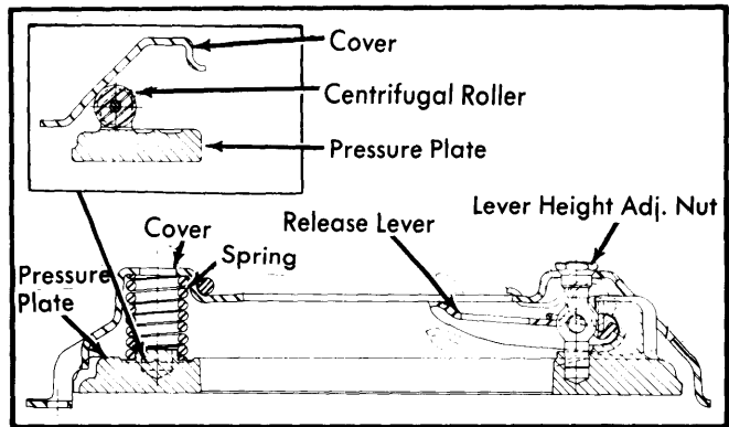
Fig. 2 Cross Sectional View of Chrysler Corp. Clutch
