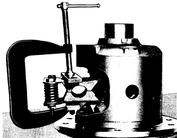
Fig. 2 Removing Preload Spring Pack (Coil Type Preload Spring)
