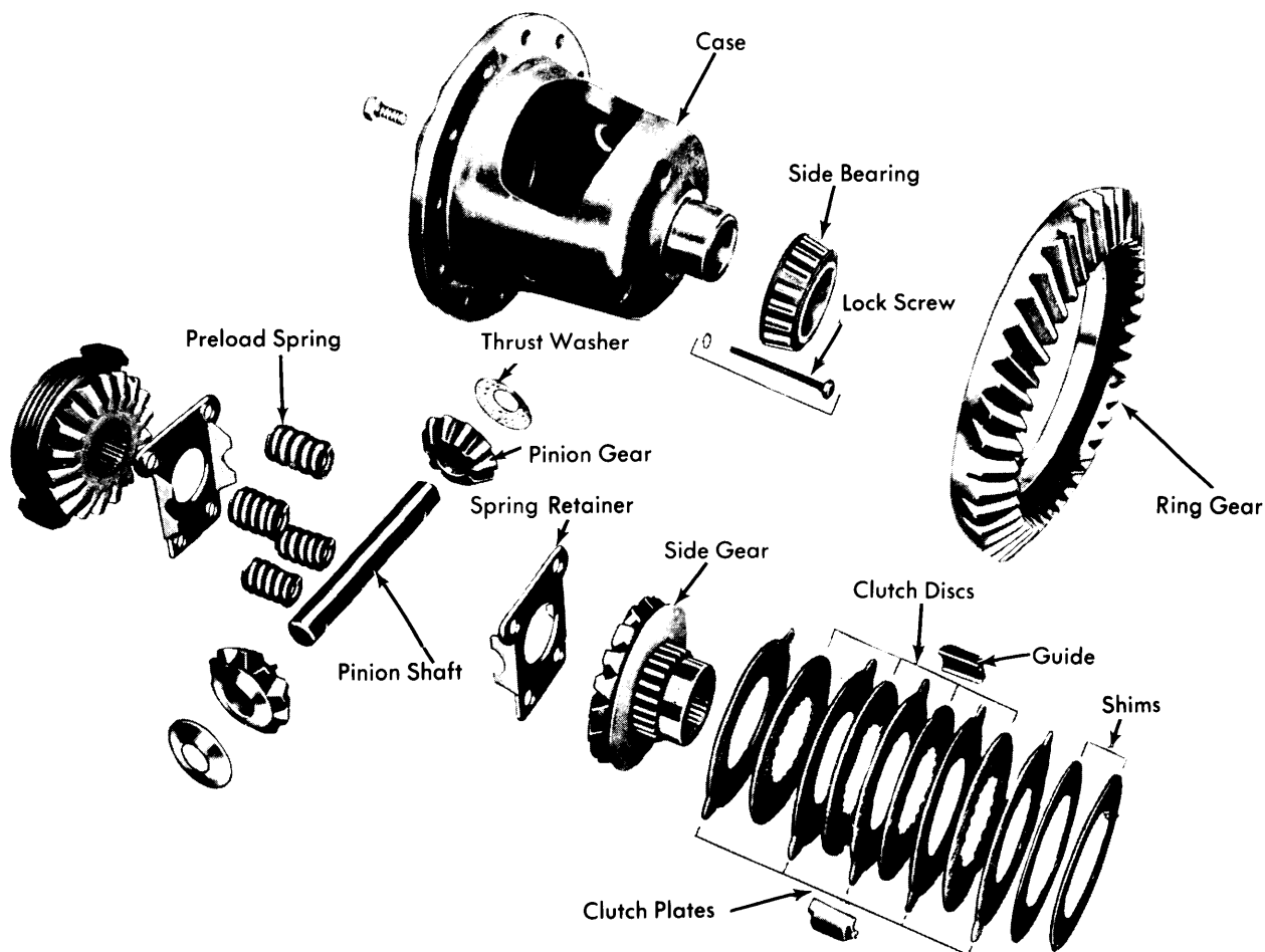
Fig. 3 Exploded View of Positraction Unit (Coil Type Preload Spring)
