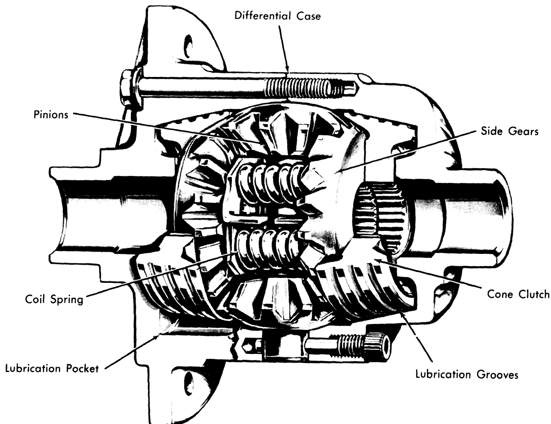
Fig. 1 Cutaway View of Chrysler Corp. Sure-Grip Differential Assembly
